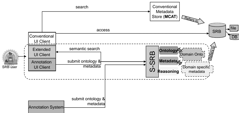
Fig. 1. S-SRB architecture
