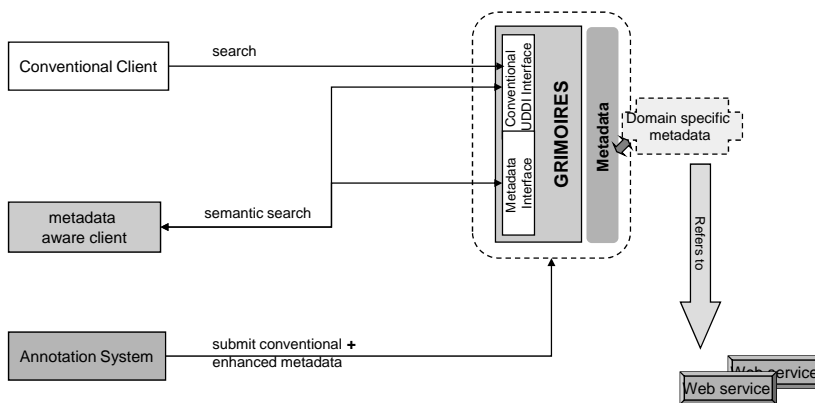
Fig. 2. GRIMORES architecture
