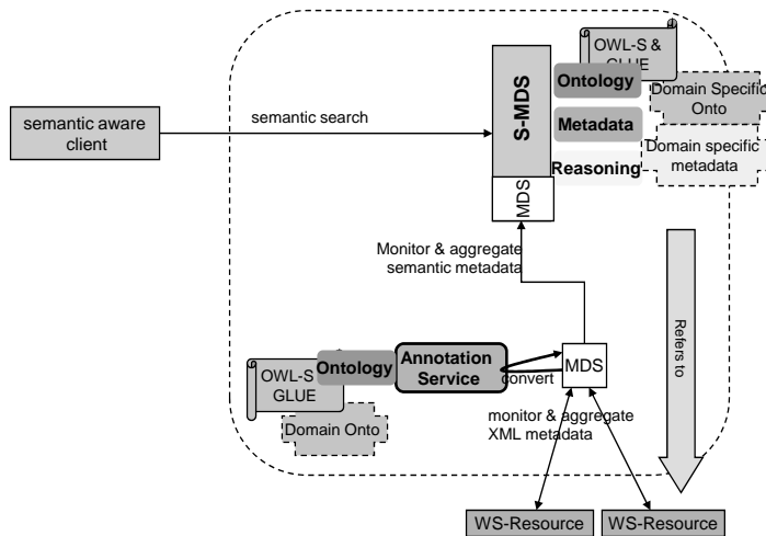
Fig. 3. S-MDS architecture
