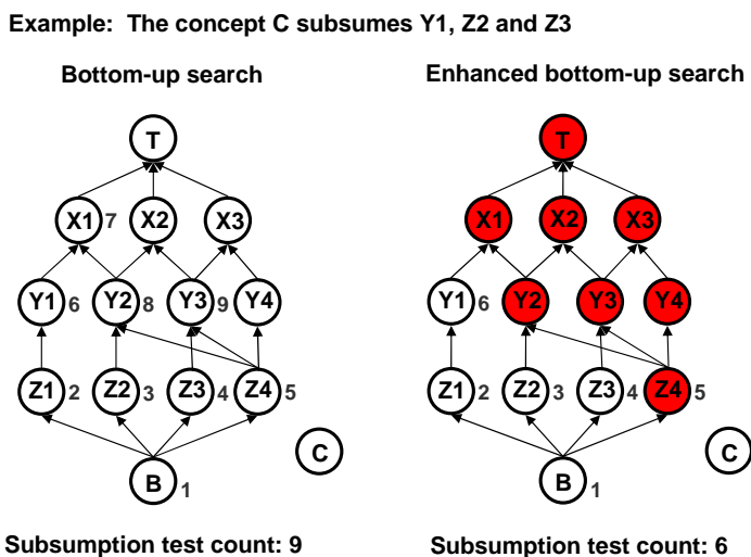
Fig. 8. Example 2 – enhanced bottom-up search processing
